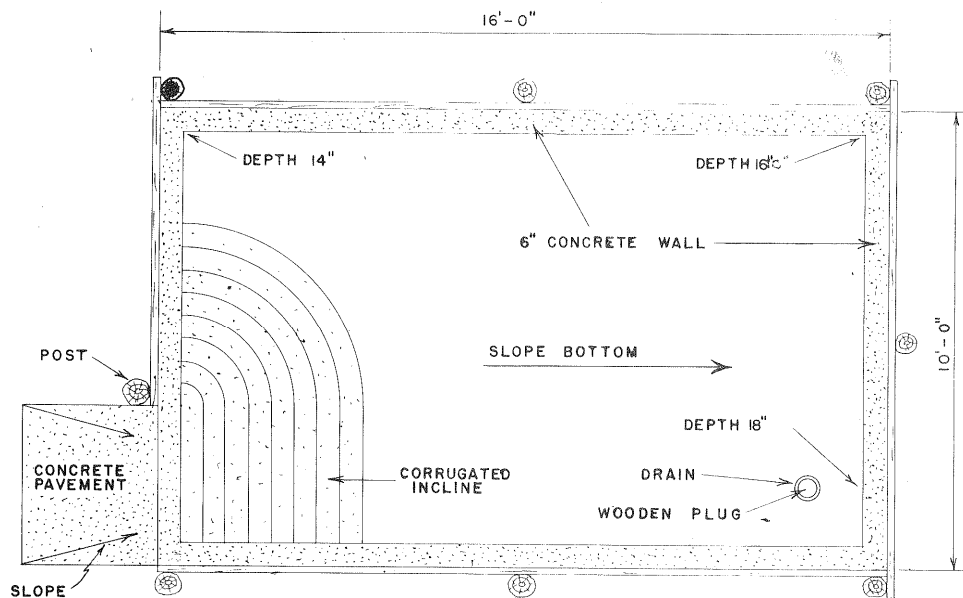
FLOOR PLAN 0 1 2 3 FT.
