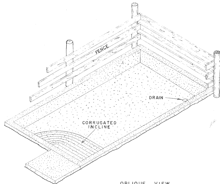
OBLIQUE VIEW 0 1 2 3 4 FT.
