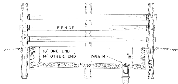
CROSS SECTION 0 1 2 3 FT.
