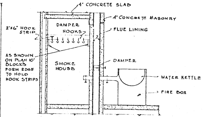
SECTION THRU SMOKE HOUSE SHOWING FLUE WITH DAMPERS TO CONTROL SMOKE
