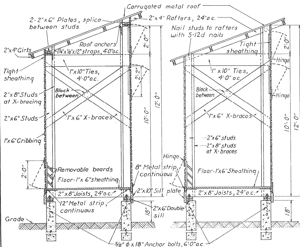
ALTERNATE FRAMING DETAIL SCALE 1/2" = 1'-0"
