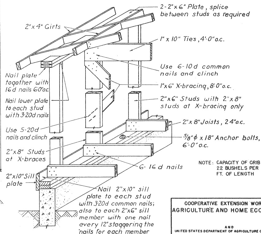
FRAMING DETAIL
