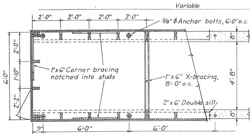
GENERAL PLAN SCALE 1/2" = 1'-0"
