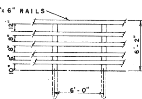
TYPICAL LINE FENCE
