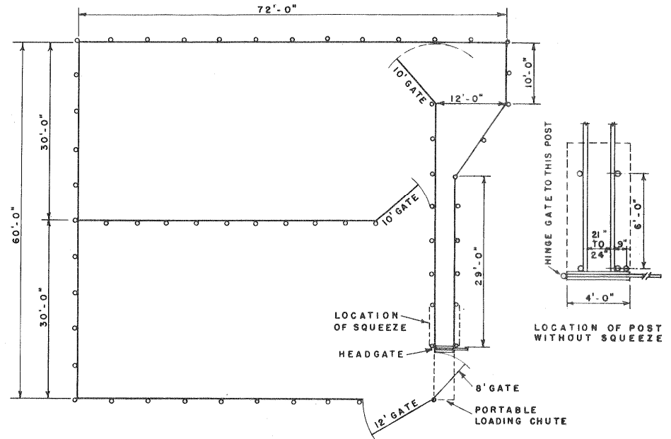
PLAN NO. 2 WITH OUTSIDE WORKING CHUTE
