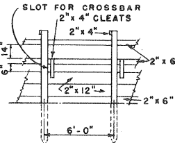
TYPICAL CHUTE
