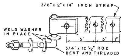
TYPICAL GATE HINGE
