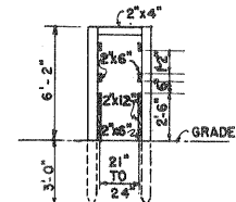
SECTION THRU CHUTE
