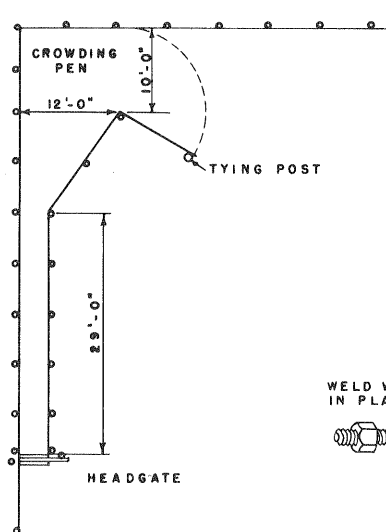
PLAN OF CHUTE IN CORNER OF PASTURE
