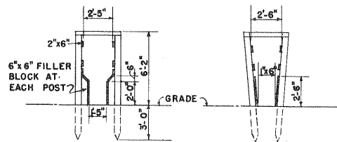
SECTIONS THRU ALTERNATE CHUTES
