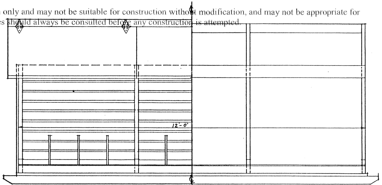
ASSEMBLY • FRONT ELEVATION • FRAMING • EAR CORN SELF FEEDER •
