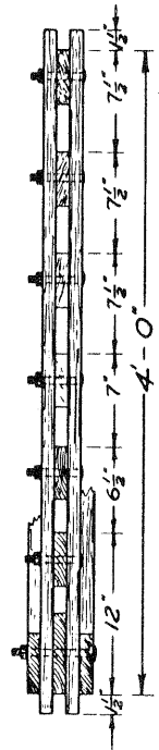
END VIEW
