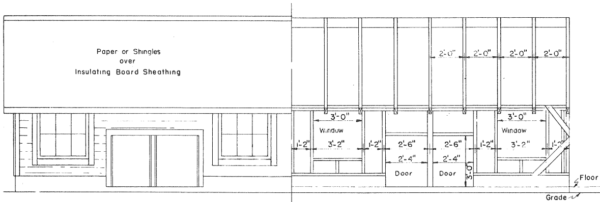
ELEVATION 0 1 2 3 4 FT.
