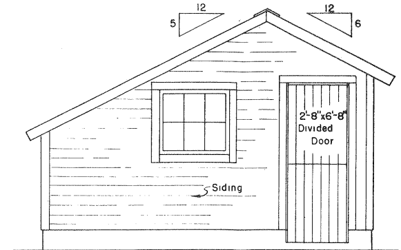
ELEVATION 0 1 2 3 4 FT.
