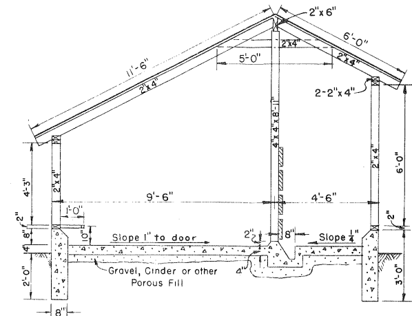
SECTION "A-A" 0 1 2 3 4 FT.
