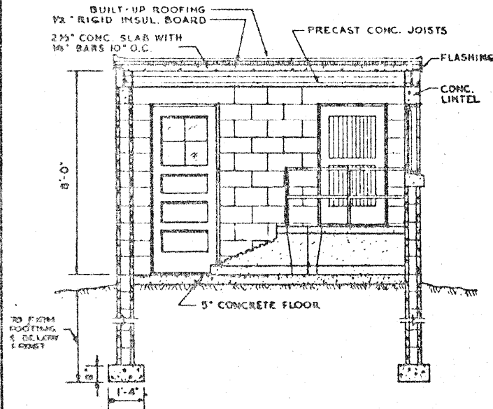
SECTION-ALTERNATE CONSTRUCTION
