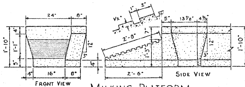
MILKING PLATFORM
