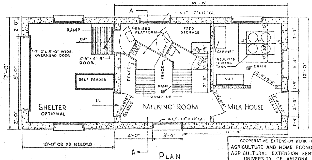
MILKING PLATFORM
