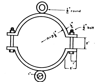
DETAIL 'C' GUY BAND (1 Required)
