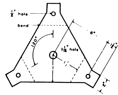
DETAIL 'A' SPIDER To be made of 1/2" plate (W.I.) (1 required)
