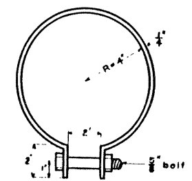
DETAIL 'B' BANDS 2 Required
