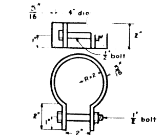
DETAIL 'D' BANDS (2 Required)
