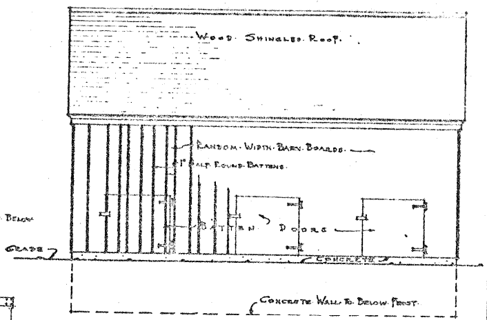
• REAR ELEVATION •
