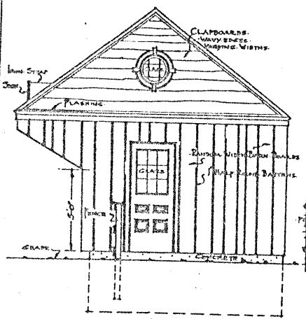
• SIDE ELEVATION •
