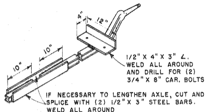
AXLE ASSEMBLY ADAPTED FROM AUTOMOBILE FRONT AXLE AND WHEEL ASSEMBLY OR OTHER DROP AXLE.
