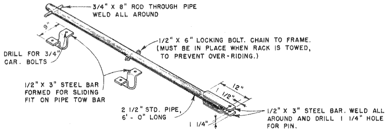
TOW BAR ASSEMBLY TO SLIDE BACK UNDER FLOOR OF RACK WHEN NOT IN USE.
