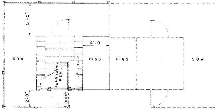
PLAN SHOWING SINGLE OR DOUBLE LAYOUT
