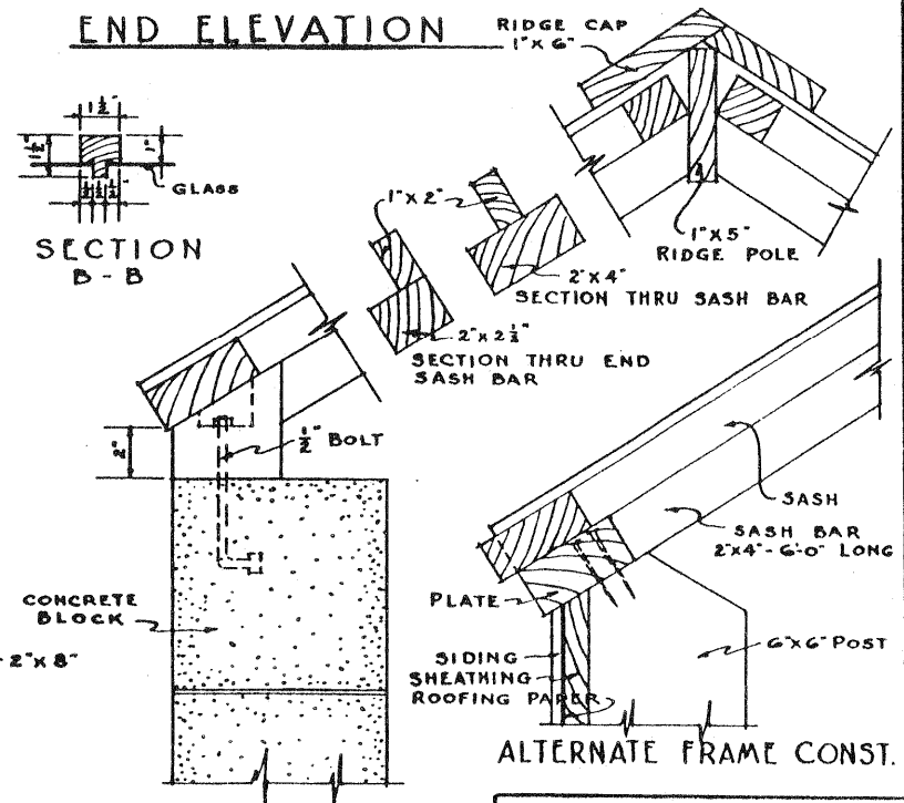
DETAILS OF EAVE & RIDGE CONSTRUCTION
