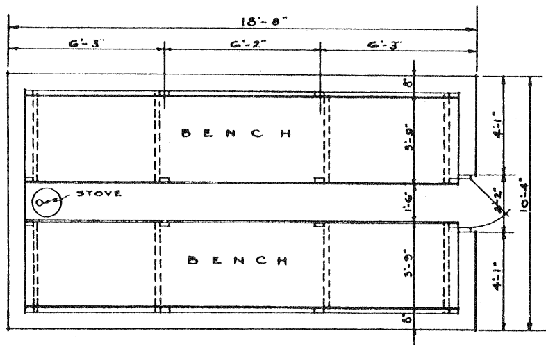
PLAN SHOWING ARRANGMENT OF BENCHES
