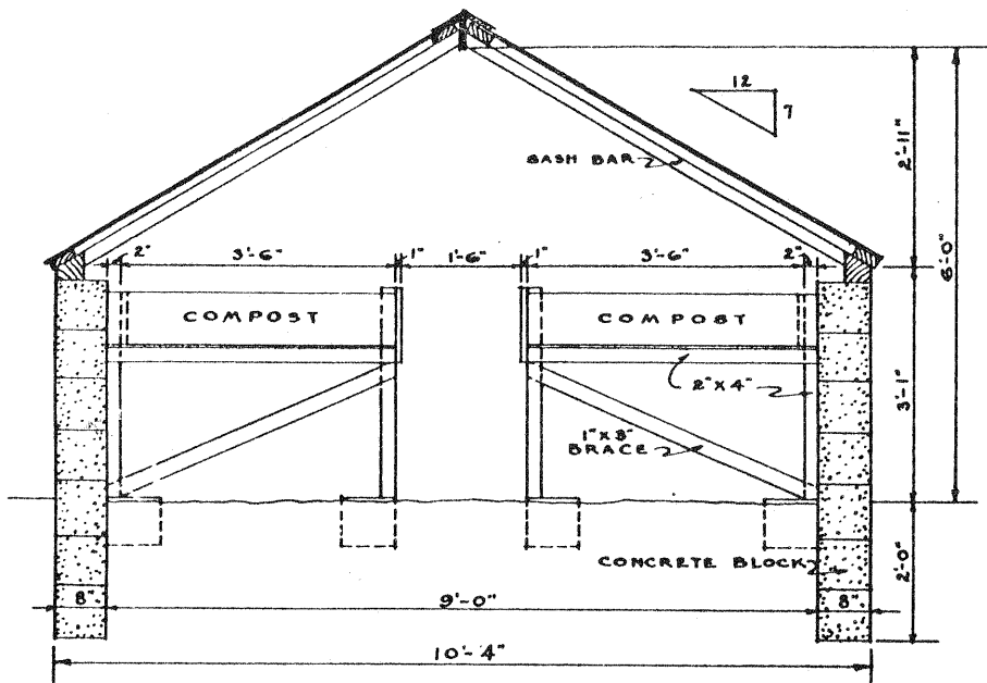
END SECTION
