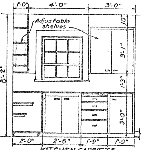
KITCHEN CABINETS Scale 1/4" = 1'-0"
